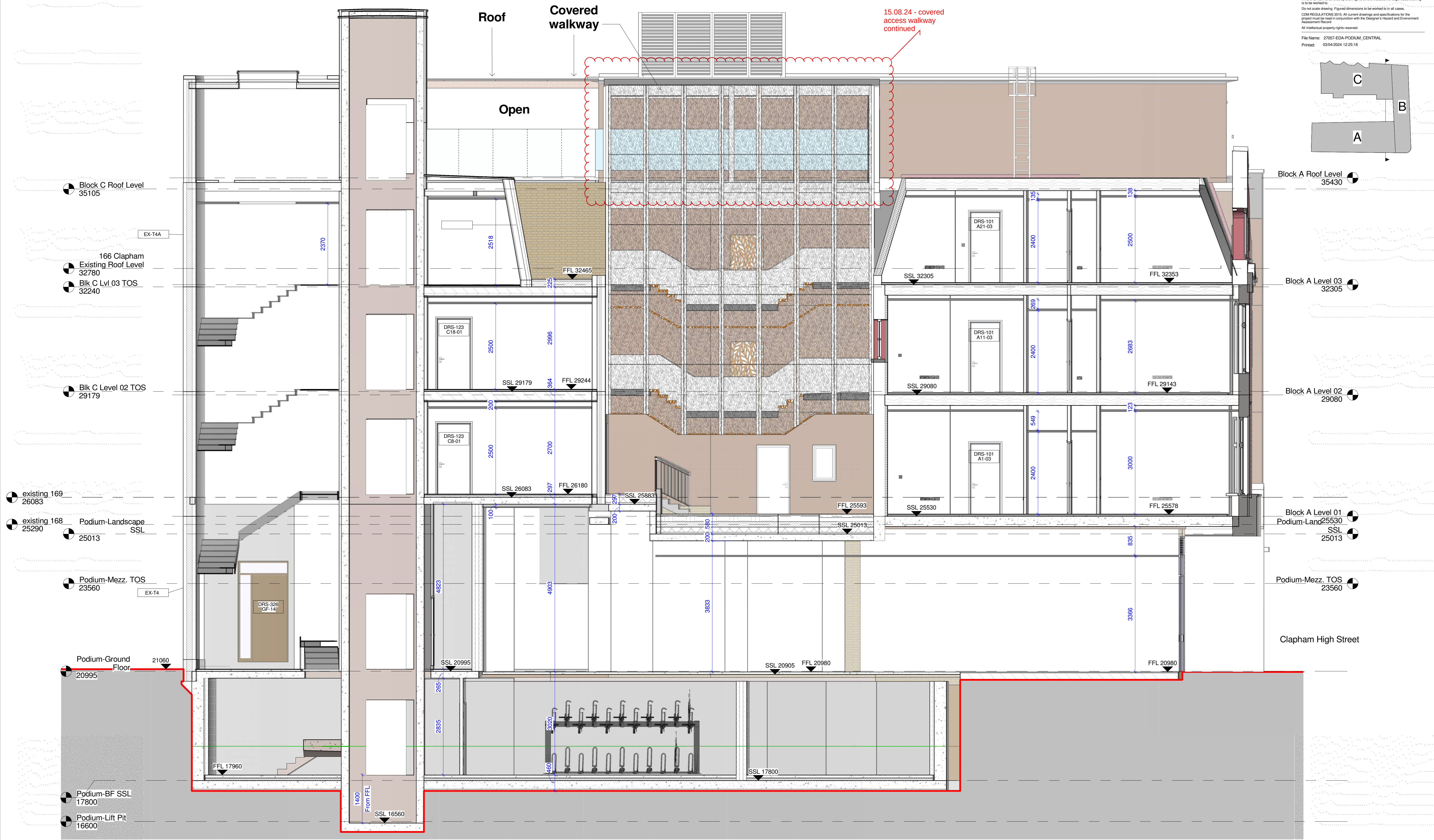
Courtyard Elevation - Block B Planning
